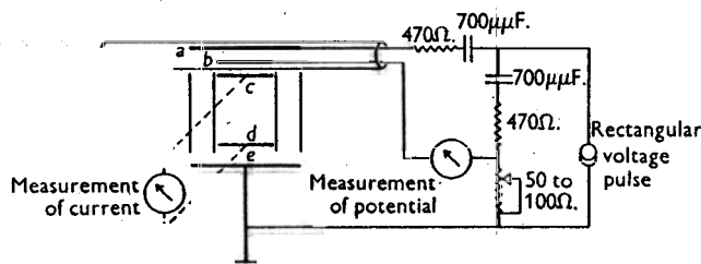
Fig. 7. Diagram of arrangement for recording response of membrane to short shock.
