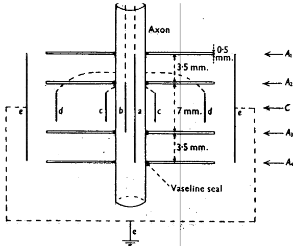
Fig. 1. Diagram illustrating arrangement of internal and external electrodes. A_1 , A_2 , A_3 and A_4 are Perspex partitions. a , b , c , d and e are electrodes. Insulated wires are shown by dotted lines. For sections through A and C , see Figs. 2 and 3.
