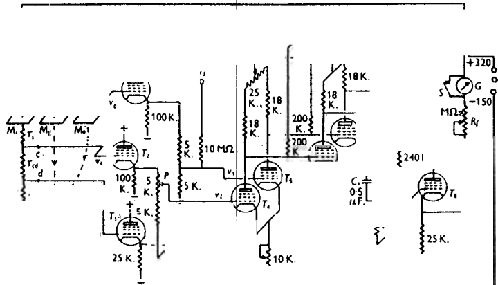
Fig. 6. Schematic diagram of feed-back amplifier. Screen resistances, grid stoppers and other minor circuit elements have been omitted. T_1, T_2, T_3 and T_8 are cathode followers; T_4, T_5, T_6 and T_7 are d.c. amplifiers. All valves were 6AK5 except T_1 and T_3 which were 1223. G is a microammeter used in setting-up. S is a switch for short-circuiting G . M_c is the membrane in the central section of the guard system. M_g , membrane in guard channels. M_o , membrane outside guard system. i_c, i_g and i_o are currents through these elements. r_{cd} , fluid-resistance used to measure current ( 74 \Omega . at 20^\circ \text{C} ). r_s , resistance in series with membrane (about 52 \Omega . at 20^\circ \text{C} ). z_{de} , impedance of large earthed electrode and sea water between d and e . Potentials are given with respect to earth.
