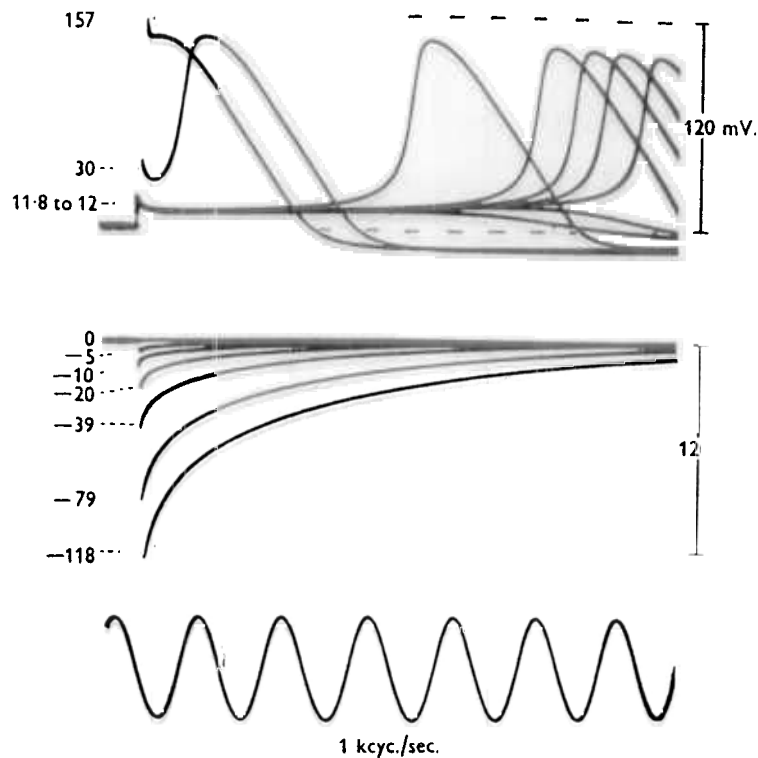
Fig. 9. Time course of membrane potential following a short shock at 6^\circ\text{C} . Depolarization shown upwards. Axon 17. The numbers attached to the curves give the strength of shock in \text{m}\mu\text{coulomb/cm.}^2 . The initial displacement in the case of the uppermost curve cannot be seen; its value was about 200 mV.
